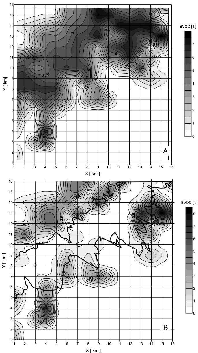
Fig. 5. Spatial distribution of total BVOC emissions (isoprene, total monoterpenes and other VOC) for the High Tatras model domain of periods: A – before windstorm, B – after windstorm (solid black line – border of damaged forest area).
