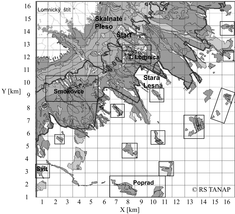
Fig. 1. The High Tatras domain definition area: square 16 km × 16 km; grid 1 km; gradate of grey color – forest vegetation before November 19, 2004 windstorm; solid grey line – border of area affected by windstorm; white color – no forest vegetation; rectangles – urban and rural settlements.
