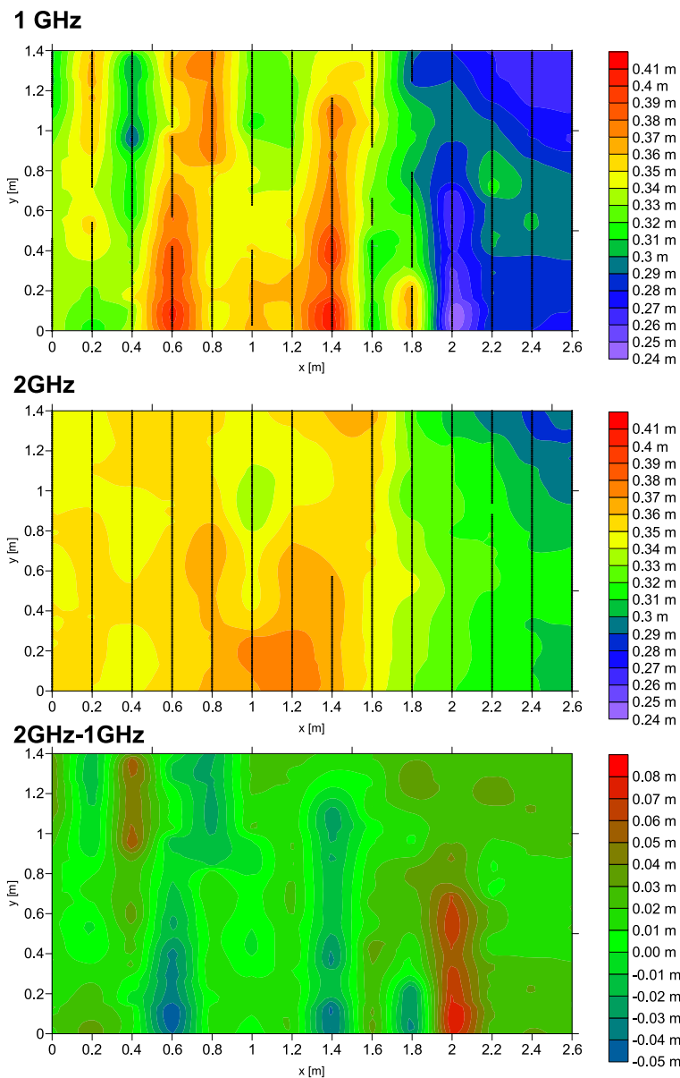
Fig. 5. Layer 2 in x -direction (Lay2X); a) result obtained by 1 GHz antenna; b) result obtained by 2 GHz antenna; c) result obtained by subtraction of 1 GHz antenna from 2 GHz antenna.
