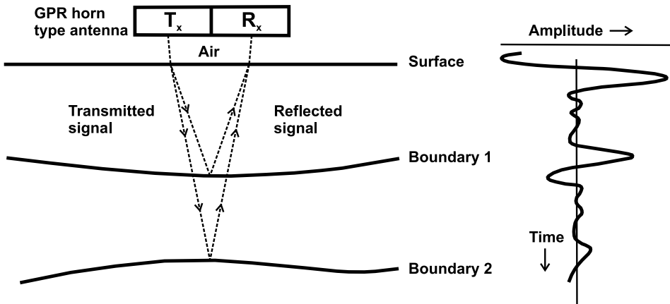
Fig. 1. Principle of GPR investigation (modified according to Matula (2013) ). T_x is transmitting antenna and R_x is receiving antenna.
