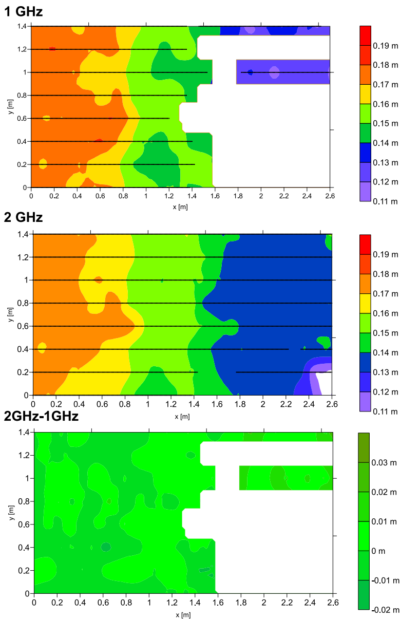
Fig. 3. Layer 1 in x -direction (Lay1X); a) result obtained by 1 GHz antenna; b) result obtained by 2 GHz antenna; c) result obtained by subtraction of 1 GHz antenna from 2 GHz antenna. White fields on maps show areas where no data are available.
