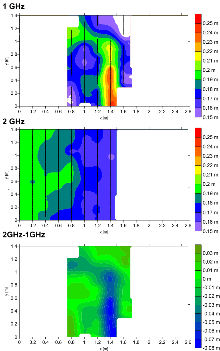
Fig. 4. Layer 1 in y -direction (Lay1Y); a) result obtained by 1 GHz antenna; b) result obtained by 2 GHz antenna; c) result obtained by subtraction of 1 GHz antenna from 2 GHz antenna. White fields on maps show areas where no data are available.
