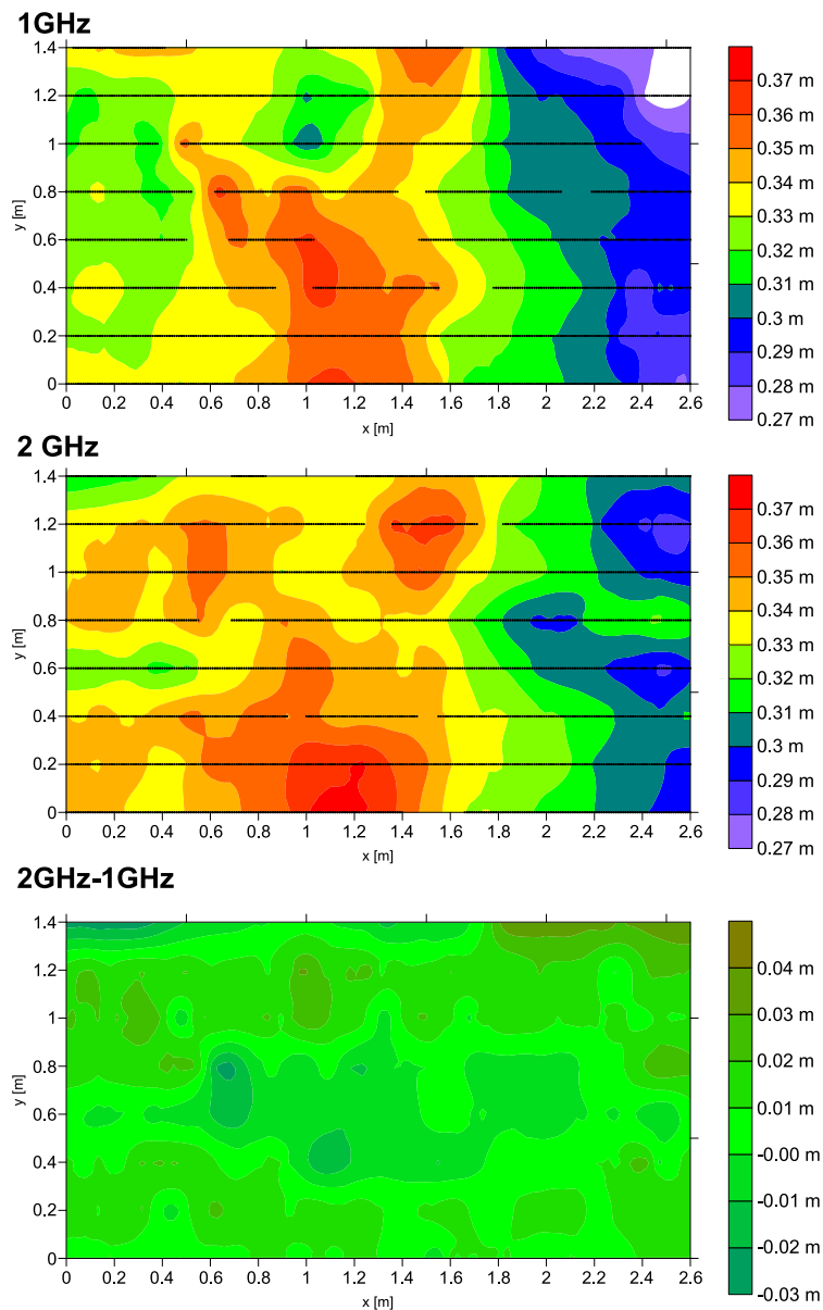
Fig. 6. Layer 2 in y -direction (Lay2Y); a) result obtained by 1 GHz antenna; b) result obtained by 2 GHz antenna; c) result obtained by subtraction of 1 GHz antenna from 2 GHz antenna.
