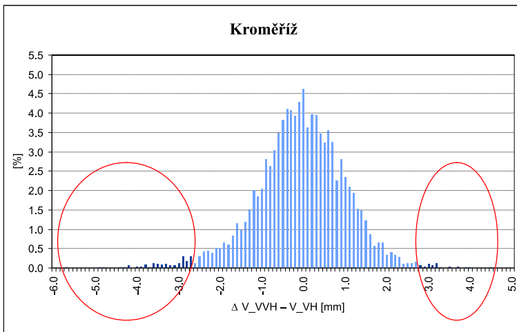
Fig. 1. Kroměříž, histogram of frequency of differences in daily evaporation between calculated data and data measured by GGI-300 during the vegetation period from May to September (1971–2000). The x -axis label symbol \Delta denotes the difference between V_{VVH} and V_{VH} in mm.
