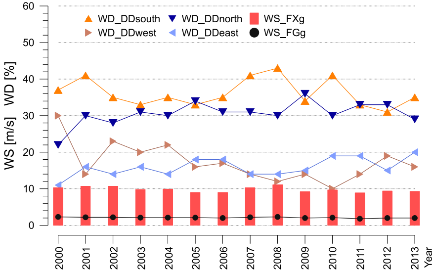
Fig. 4. Annual variation of WS – wind speed and WD – wind direction characteristics.
