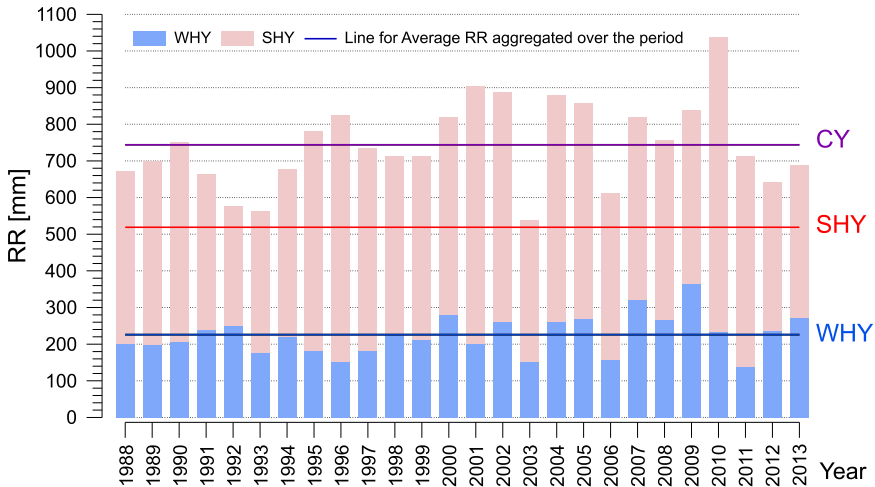
Fig. 3. Annual precipitation amount aggregated over SHY-summer half year; WHY – winter half year; calender year – CY.
