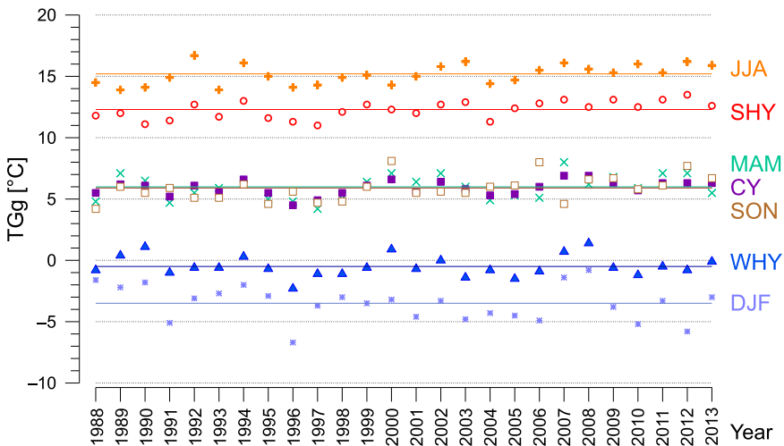
Fig. 1. Annual variation (points) and seasonal average (lines) of mean air temperature TGg.
