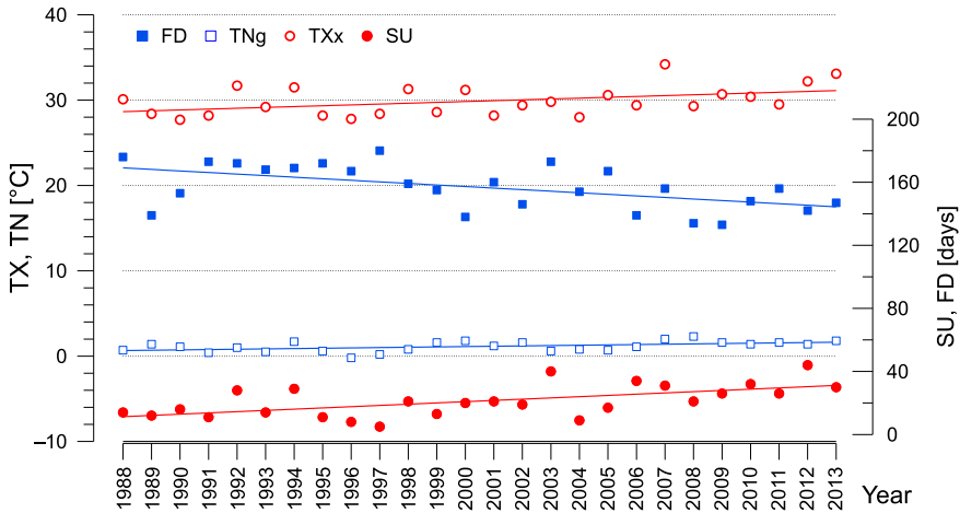
Fig. 2. Annual variation of extreme air temperatures (points) and statistically significant linear regressions (lines): TXx – daily maximum; TNg – mean of daily minimum; SU – number of summer days; FD – number of frost days.
