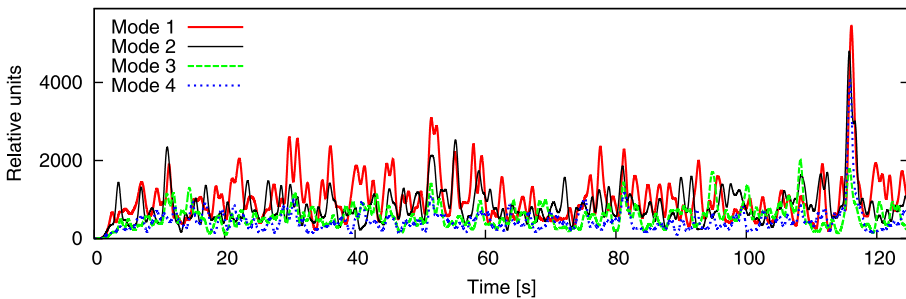
Fig. 4. The smoothed amplitude residuals for the first four SR modes of the signal in Fig. 3. Horizontal axis in seconds, vertical in relative units. Smoothing was made through moving half-cosine window 2.5 s wide.
