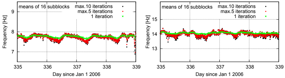
Fig. 10. Results of the 1st and 2nd mode demodulation of 327.68-second measured sequence calculated as a mean of all 16 sub-blocks. Points of different type and colors differentiate between demodulation procedure runs, which were limited to either 1, 5 or 10 iterations. The axes and the scale are the same as in Fig. 9. Naturally, these values are less scattered than frequencies determined for sub-blocks.
