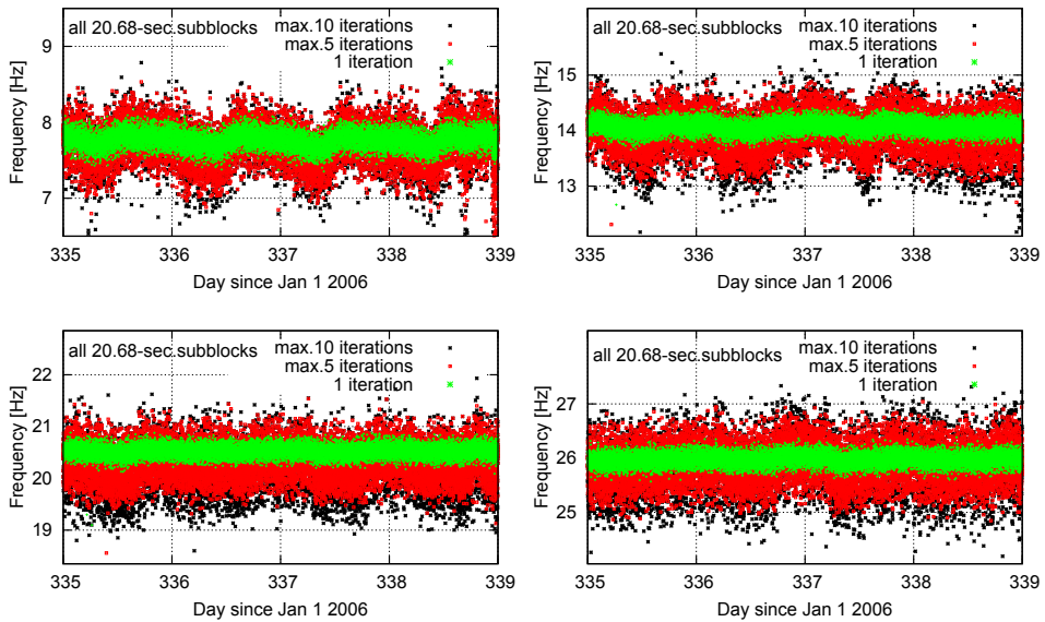
Fig. 9. The results of complex demodulation of the four Schumann modes from December 1–4, 2006. For every day, 3840 points are given (240 data blocks each day are divided into 16 sub-blocks and every sub-block was processed independently). Points of various types and colors differentiate between demodulation procedure runs, which were limited to either 1, 5 or 10 iterations.
