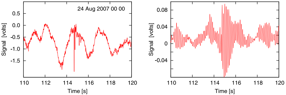
Fig. 5. ( left ) A selected part of unfiltered signal from Fig. 3 and ( right ) the same signal but prefiltered with the 1st Schumann mode filter ( f_0 = 7.80 Hz). The time interval covers the signal from 110 s to 120 s after the data block beginning. Horizontal axis is in seconds, vertical axis in left graph is in volts at true receiver output. The vertical axis on the right represents the receiver output diminished by constant attenuation of the band-pass filter. Note the onset of a transient (Q-burst) at 114.67 s, which is consistent with maxima of amplitude residuals of all modes in Fig. 4.
