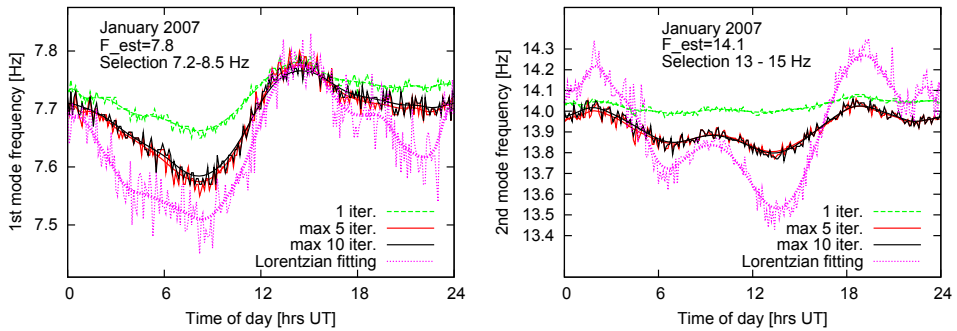
Fig. 12. Daily variations of the 1st and 2nd Schumann mode resonance frequency averaged over one month (January 2007). Individual curves show daily variation determined by complex demodulation procedures, when number of iterations was limited to 1, 5, and 10, respectively, and by the Lorentz function fitting. The initial guess value of f_{est} was taken 7.80 Hz and 14.1 Hz for the 1st and 2nd mode, respectively. Results of sub-blocks outside a reasonable interval of 7.2–8.5 Hz and 13–15 Hz have been discarded.
