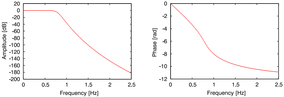
Fig. 6. Amplitude ( left ) and phase ( right ) response of the low-pass demodulation filter. Horizontal axis is frequency in Hz, vertical axis is the amplitude transfer function in dB and unwrapped phase in radians, respectively.
